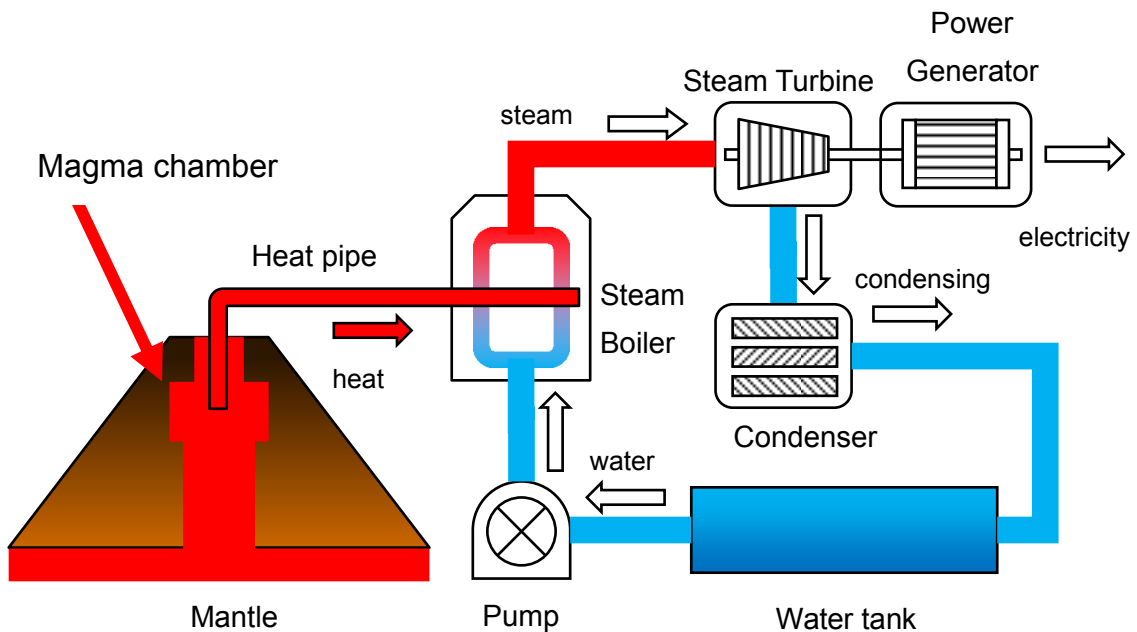
Figure Magma power plant using the conventional steam turbine
